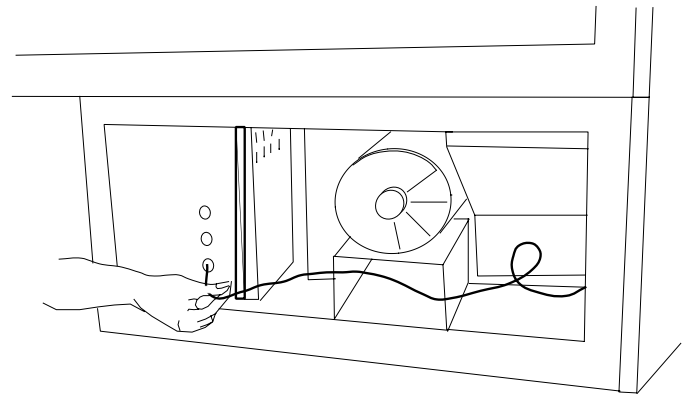
Figure 2 - Placing the Thermocouple Leads
