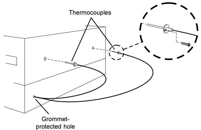
Figure 1 - Thermocouple Installation Locations
