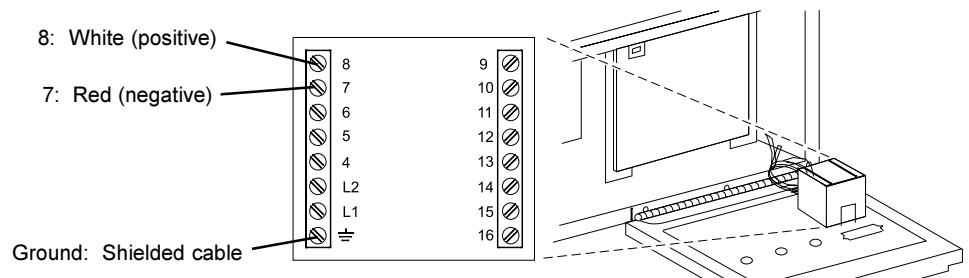
Figure 3 - Thermocouple Lead Connections
